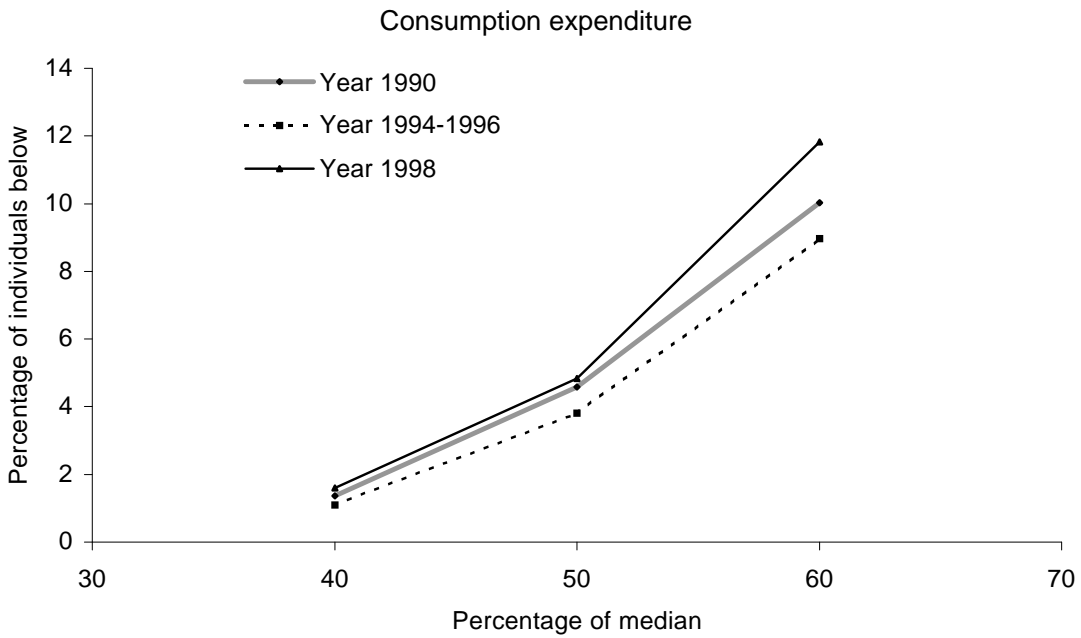
Figure 5: First-Order Dominance (FOD) from median
